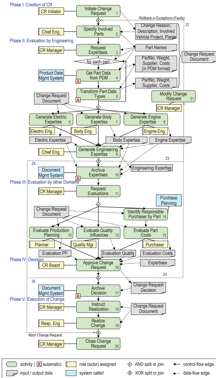
Figure 4: Process Model of a Change Request (CR)
