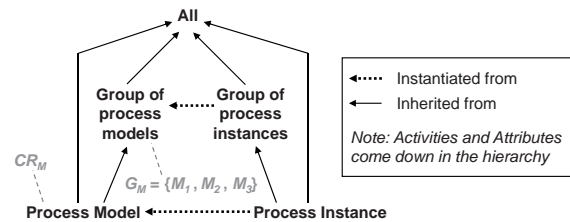
Figure 14: Objects' Hierarchy
