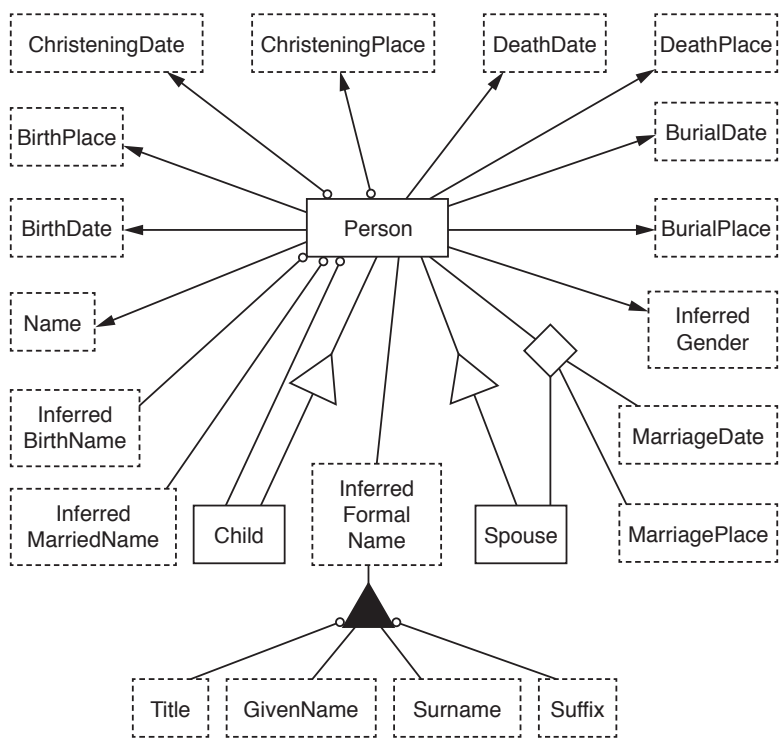
Figure 19: Ontology with Inferred Object and Relationship Sets
