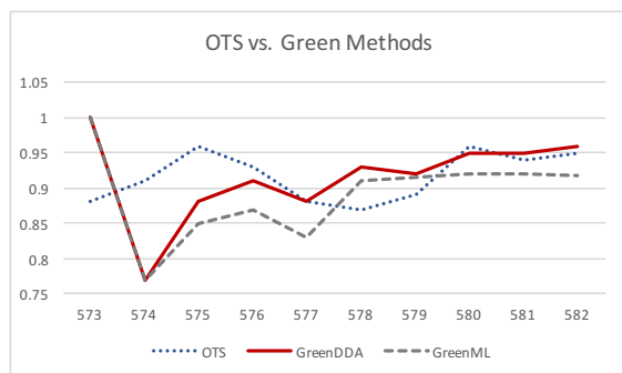
Figure 30: OTS vs. Green Methods: F-measure Annotation Results for a 10-page Range
