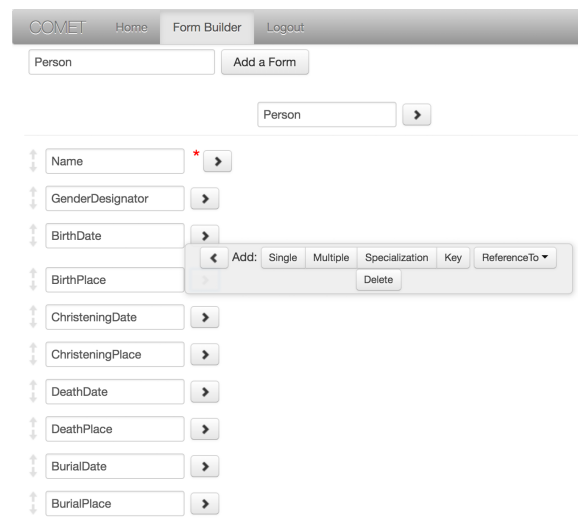
Figure 6: Form Creation and Ontology Induction
