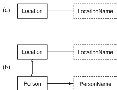
Figure 22: Location Ontology
