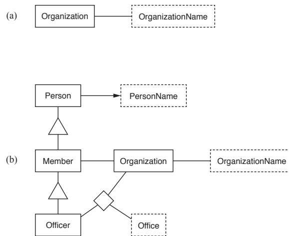
Figure 23: Organization Ontology
