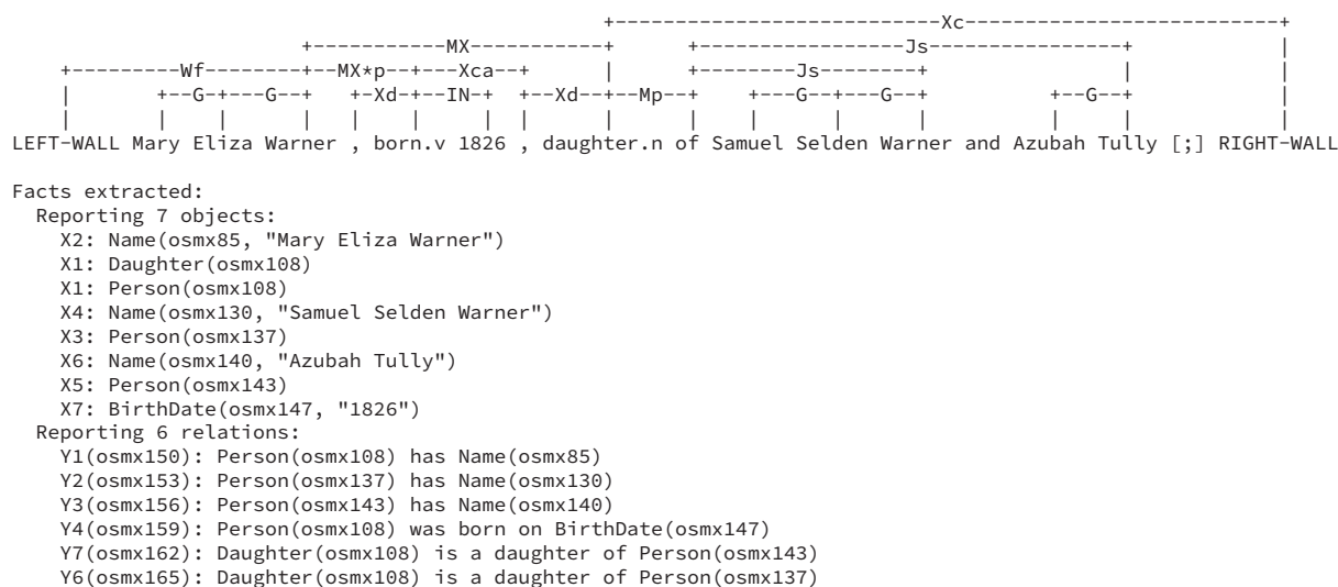
Figure 14: OntoSoar Syntax Analysis (top) and Semantic Analysis (bottom)
