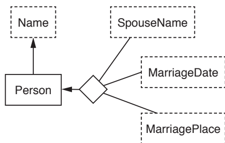
Figure 8: Couple Ontology
