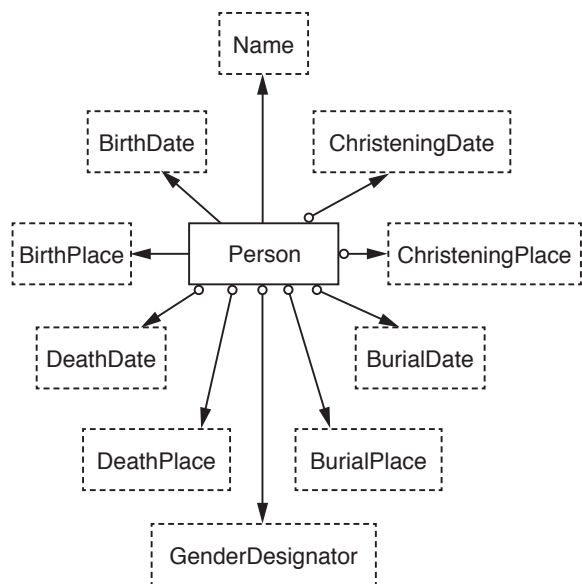
Figure 7: Person Ontology
