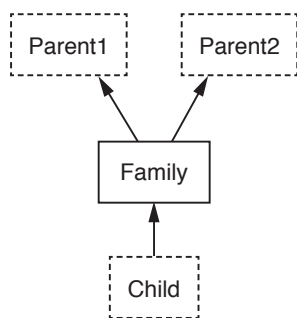
Figure 9: Family Ontology
